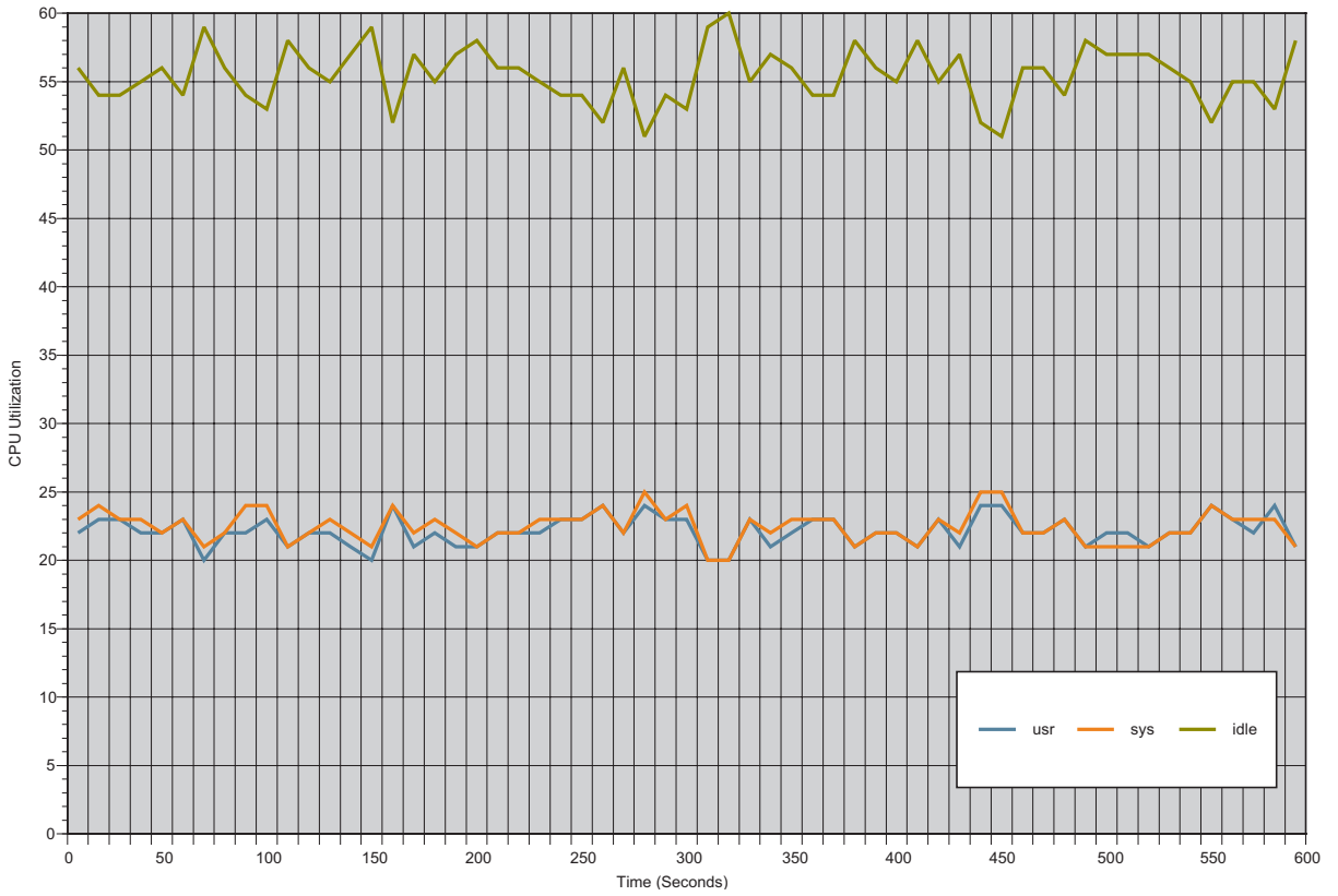
Figure 6. CPU utilization for 1,750 concurrent users with XCache enabled
