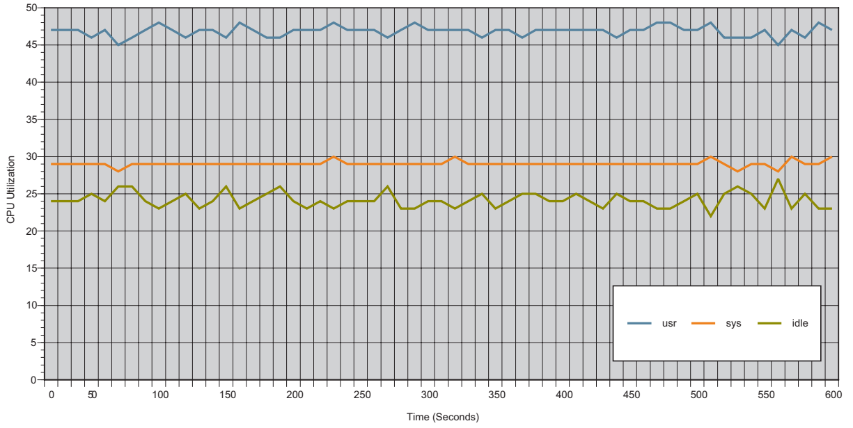
Figure 5. CPU utilization for 1,750 concurrent users with XCache disabled
