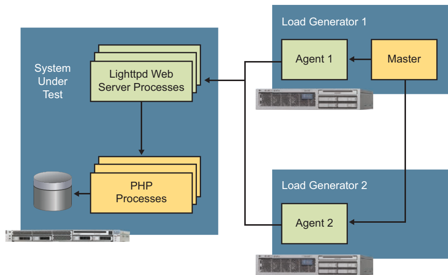
Figure 2. Configuration topology
