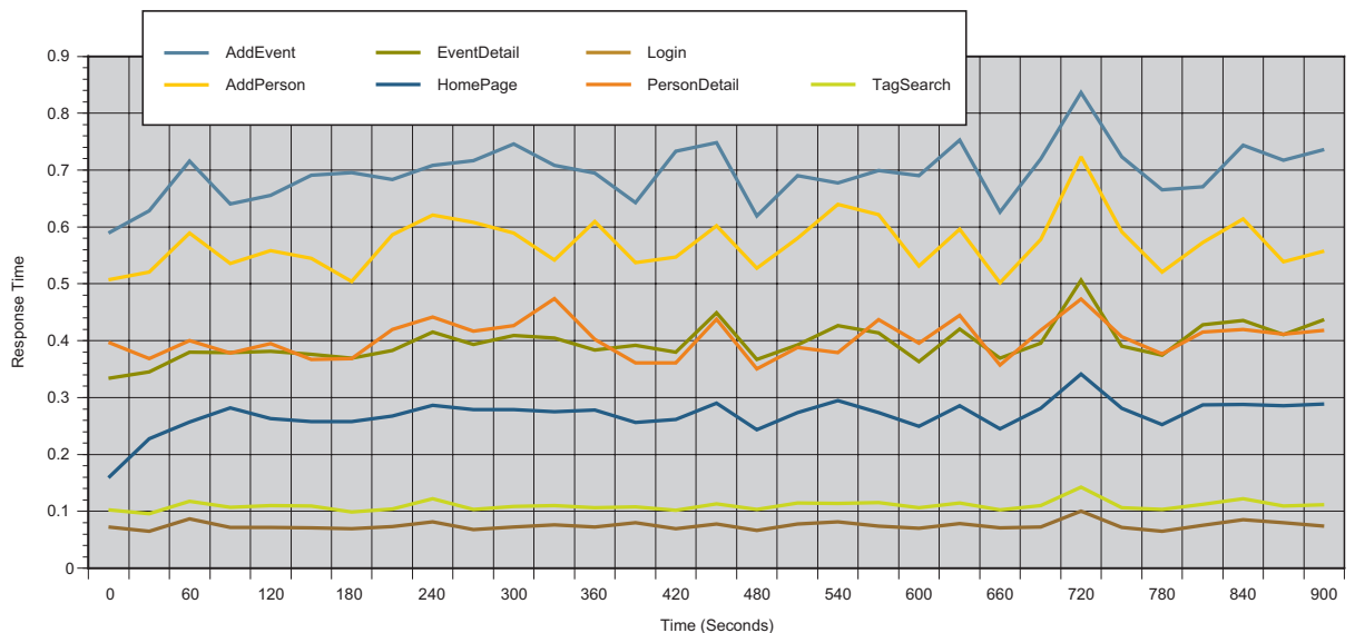
Figure 4. Response time for 1,750 concurrent users with XCache enabled
